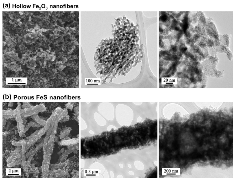
Figure 6 Morphologies of (a) hollow \text{Fe}_2\text{O}_3 nanofibers and (b) porous FeS nanofibers after 100 cycles.
