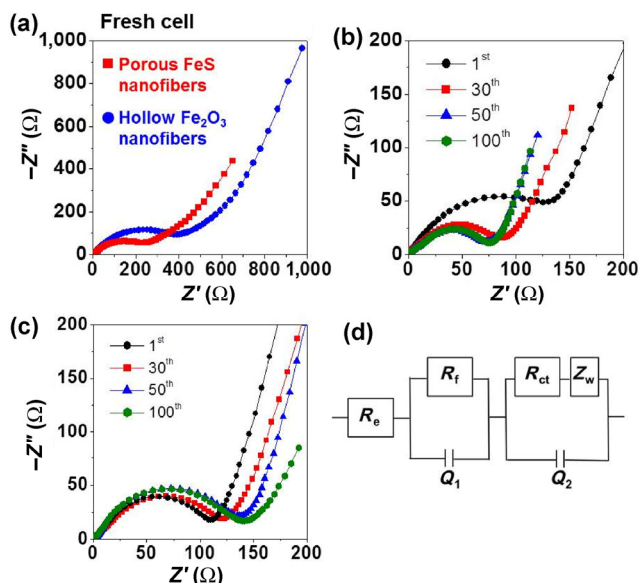
Figure 5 Nyquist impedance plots of the porous FeS and hollow \text{Fe}_2\text{O}_3 nanofibers: (a) Nyquist impedance plot of the nanofibers before cycling, (b) Nyquist impedance plots of the porous FeS nanofibers after cycling, (c) Nyquist impedance plots of the hollow \text{Fe}_2\text{O}_3 nanofibers after cycling, and (d) equivalent-circuit model used for alternating-current impedance fitting.
